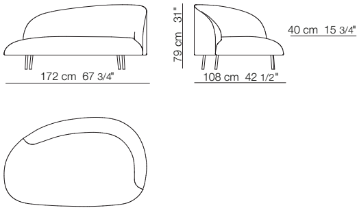
Divano / Base in metallo Sofa / Metal base
