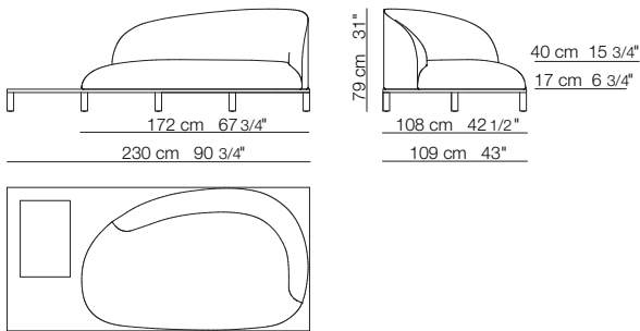
Divano / Base in legno Sofa / Wooden base
