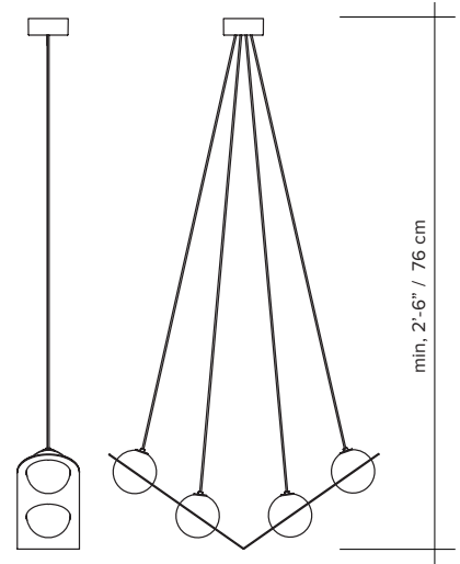
angled wires
