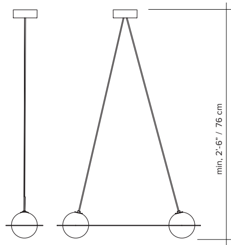
angled wires
