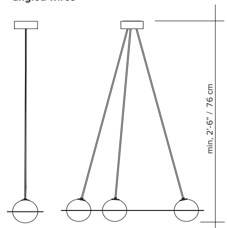
angled wires
