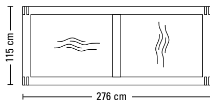
VNU I - top view
