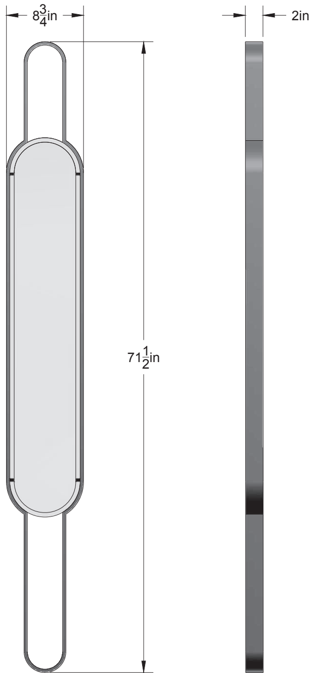
FRONT VIEW
