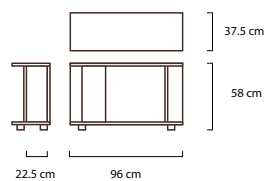
Cabinet
