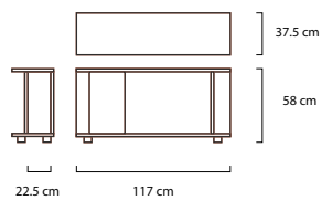
Cabinet
