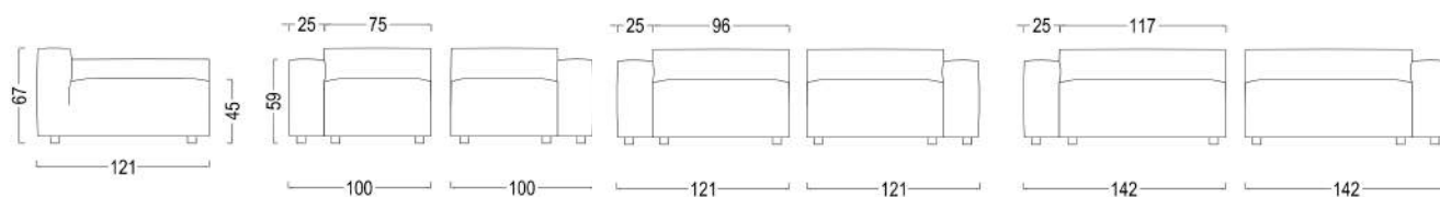
Deep lateral unit with low arm
