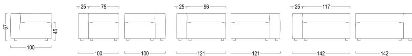
Undeep lateral unit with high arm
