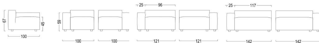
Undeep lateral unit with low arm
