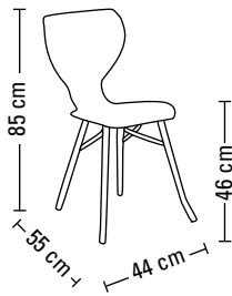
Tulipani - front view
