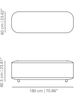
CO180H bench 180H
