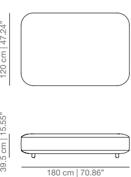
CO180H bench 180H
