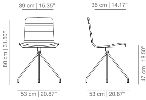
KL4PUB four star swivel base
