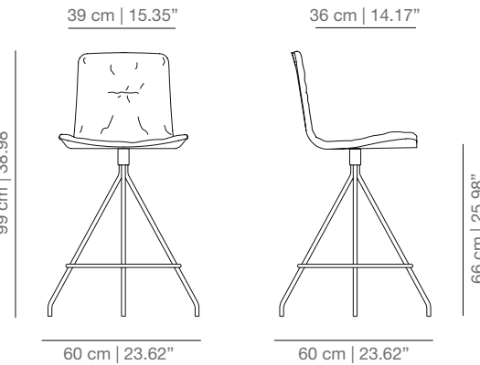
KLTCOTS swivel counter stool
