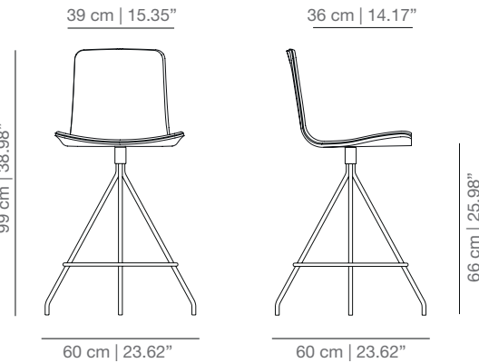
KLTCOT swivel counter stool
