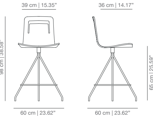
KLTCO_R swivel counter stool
