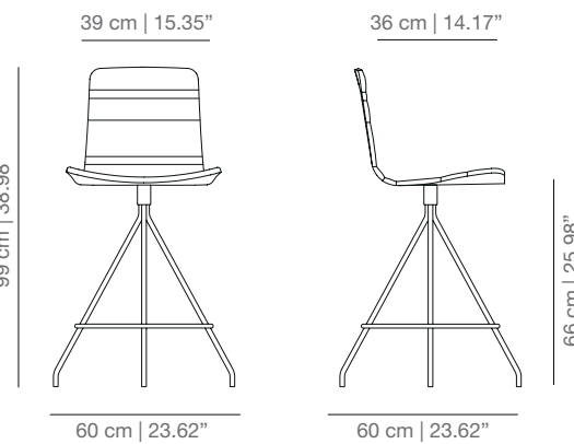
KLTCOB swivel counter stool
