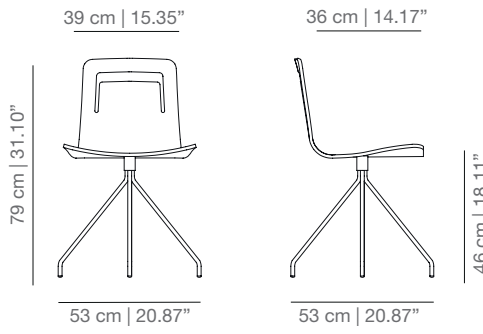
KL4PU_R four star swivel base
