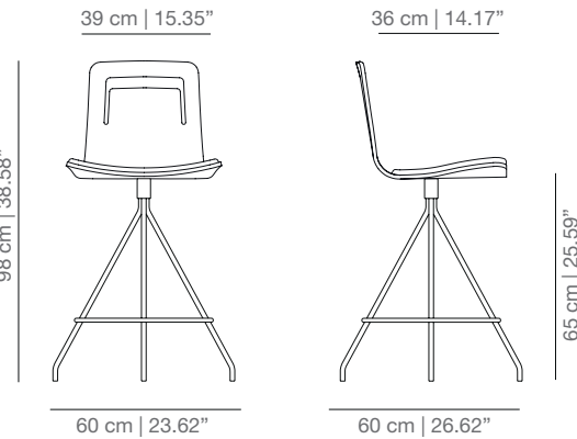
KLTCO_CR swivel counter stool
