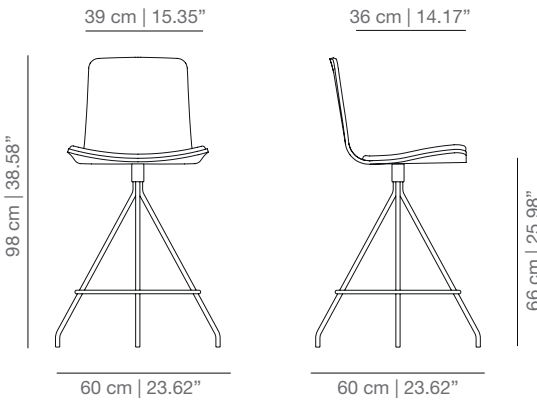
KLTCO_C swivel counter stool base without handle
