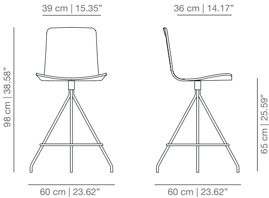
KLTCO swivel counter stool
