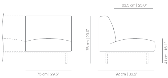
SISMP - MEDIUM BACK MODULE
