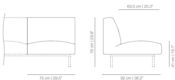
SISMP - MEDIUM BACK MODULE
